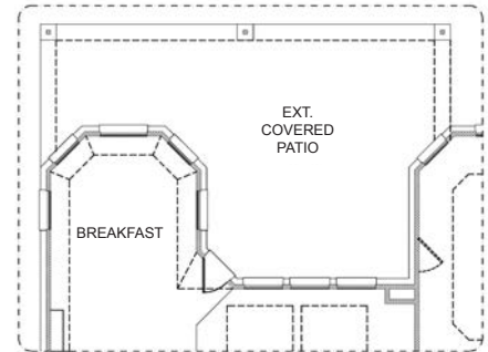
OPTIONAL EXT. COVERED PATIO
