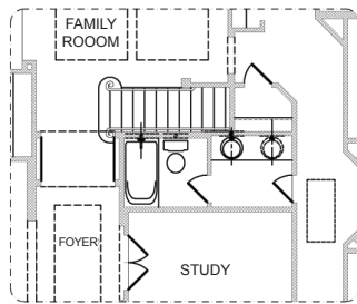
FIRST FLOOR W/ OPTIONAL BONUS ROOM
